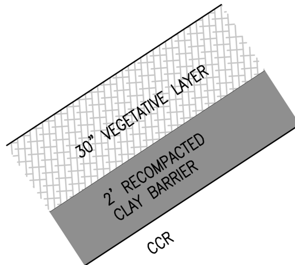
Figure 3-1 Final Cover System
